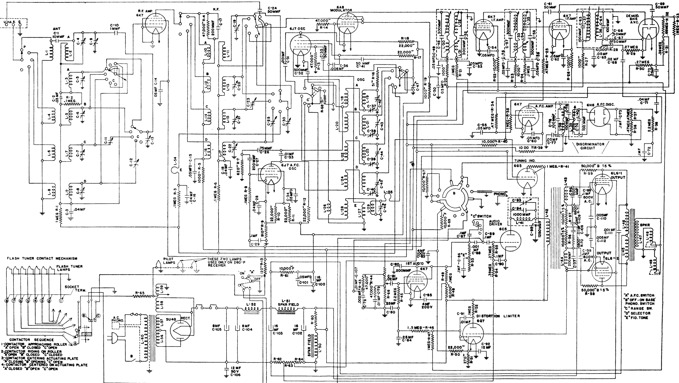
Fig. 2. Schematic Circuit.
